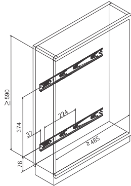
Single side mounting for 150 mm & 200 mm with KA telescopic runner
