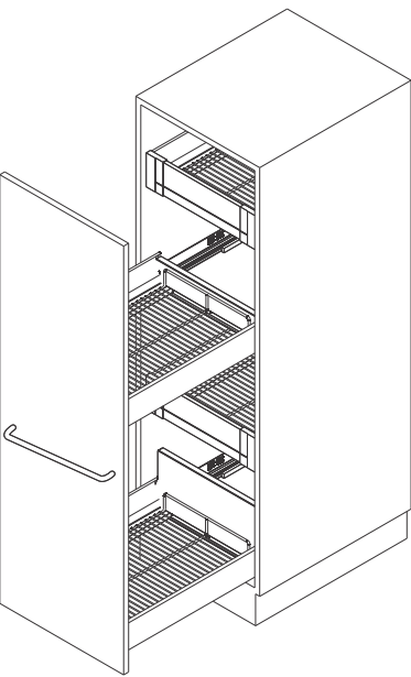
For carcase width 450 mm
