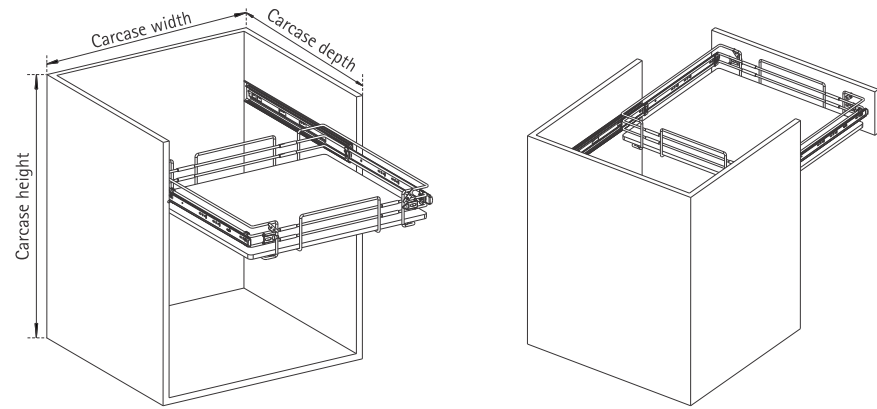
4. Check alignment with Carcase 5. Final assembly, basket fixed to fascia
