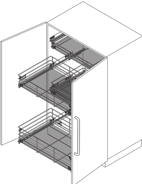
For carcase width 900 mm
