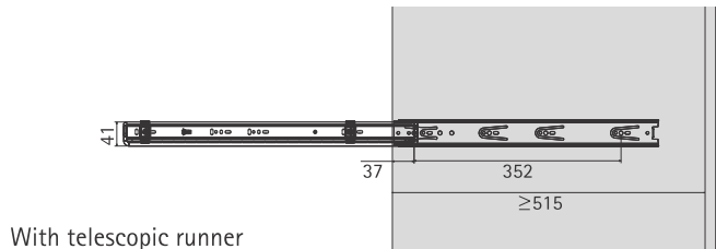
With telescopic runner
