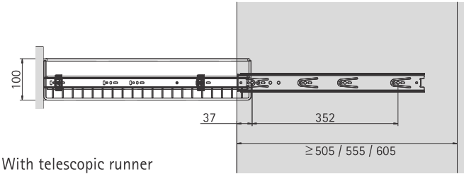
With telescopic runner
