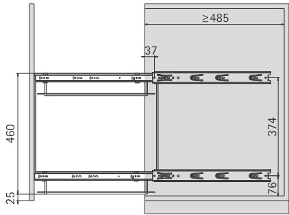
With KA telescopic runner
