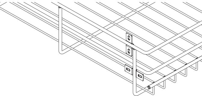
Position of Fascia attachment
