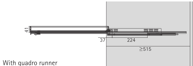
With quadro runner
