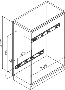
Single side mounting for 150 mm & 200 mm with KA telescopic runner Diagonal mounting for 300 mm with KA telescopic runner
