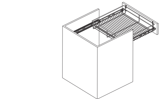
5. Final assembly, basket fixed to fascia
