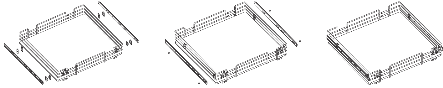
1. Align Components 2. Attach clips 3. Fix runner with clips
