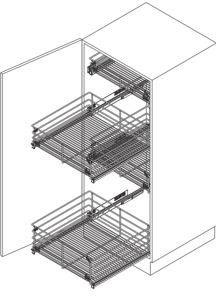
For carcase width 600 mm
