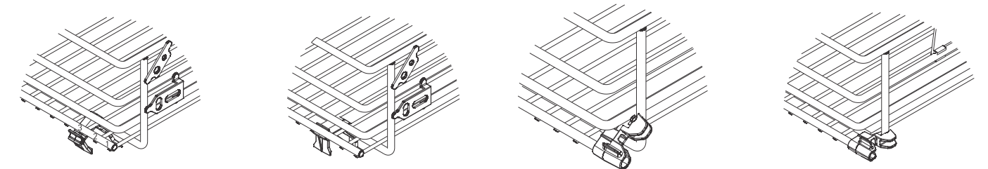
1. Push Clip-1 in third gap & rotate to fix it 2. Insert Clip-2 to back end of basket & rotate to fix it 3. Fix Clip 1 & Clip 2 to basket front & rear ends 4. Place basket over Quadro runner & fix it 5. Final assembly, basket fixed to fascia
