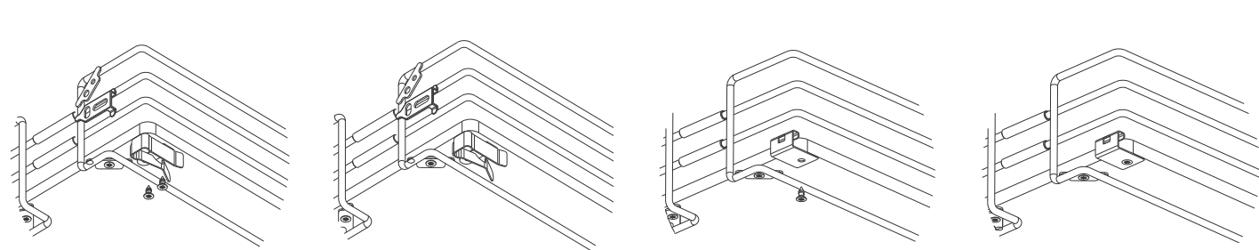
1. Fix front clip with the help of screws 2. Fix rear clip with the help of screws
